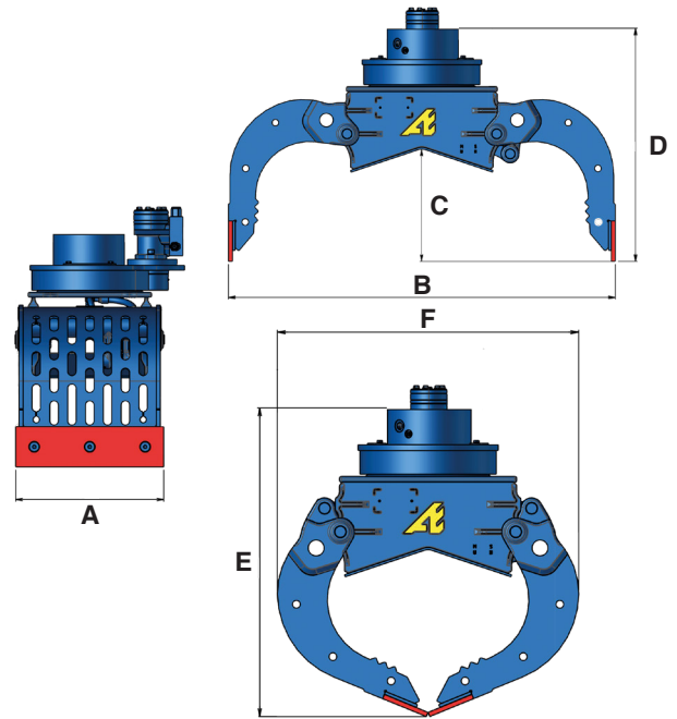
View of a S230G or S250G
