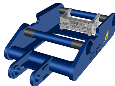
Suspension link without second link
