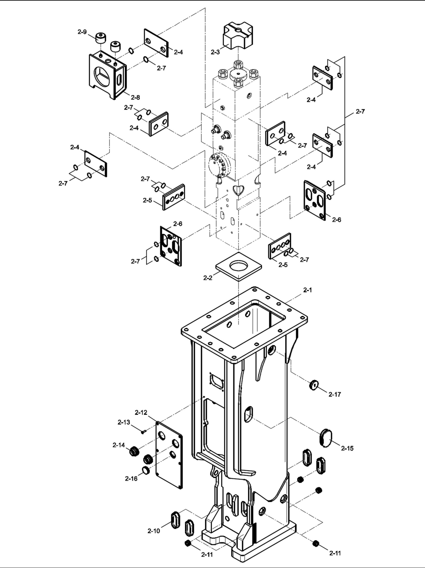
Exploded view
